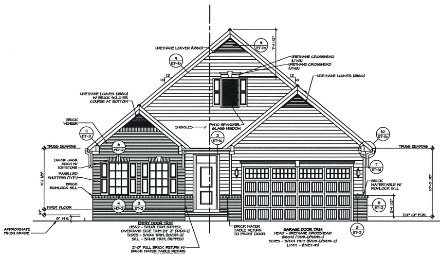
3 FRONT ELEVATION "A" SCALE: 1/4" = 1'-0" PARTIAL BRICK VENEER FRONT "500" THO CAR FRONT ENTRY GARAGE "600"
