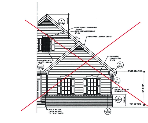
4 PARTIAL FRONT ELEVATION SCALE: 1/4" = 1'-0" PARTIAL BRICK VENEER FRONT "500" THO CAR SIDE ENTRY GARAGE "600"
